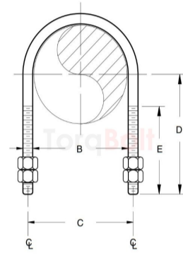
ASTM A453 Grade 660 U Bolt
