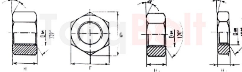
Dimensions of Hex Nuts With Metric Coarse and Fine Pitch Thread
