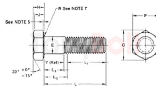
Dimensions of Heavy Hex Bolts
